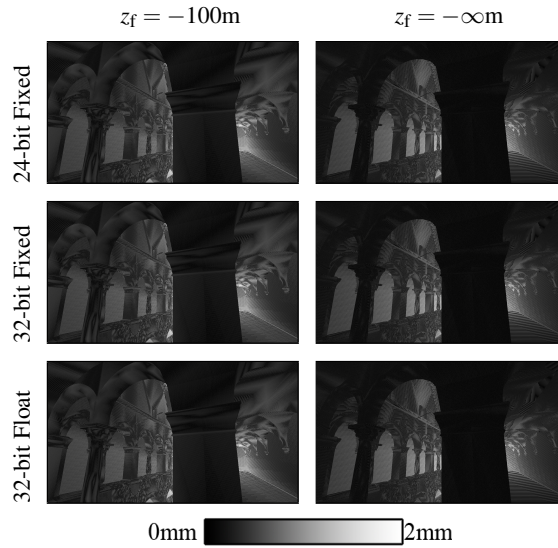
Figure 3: An infinite far plane impacts recovered z accuracy more than depth buffer format at 24-bit or higher precision.
