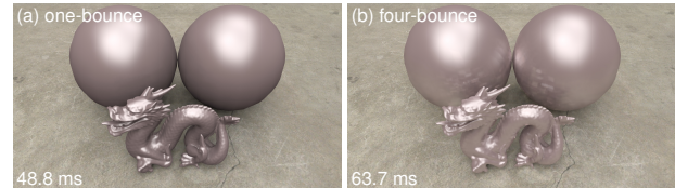
Figure 12: Rendered images by path tracing via global ray-bundles (204 k triangles scene, 55 ray-bundles per frame). Multi-bounce is computed in a time efficient manner.
