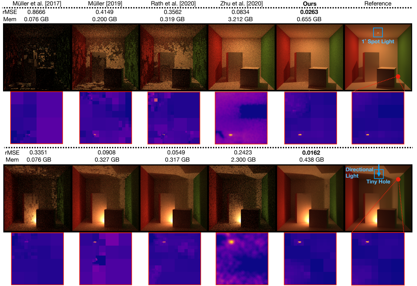
Fig. 3. Extreme conditions. We compare our method with previous path guiding methods, running with equal time, on two Cornell Box scenes that have two different extreme light transport settings. We turn on the next event estimation for all methods in this experiment. Previous methods utilize either path samples [Müller et al. 2017; Müller 2019; Rath et al. 2020] or photons [Zhu et al. 2020b] as input for path guiding, which cannot work well on both cases at the same time. In the first row, the scene is illuminated by a very small 1^\circ spotlight (facing upwards) located very close to the roof. This setting is extremely hard for path-based methods [Müller et al. 2017; Müller 2019; Rath et al. 2020] since the light is hard to connect to; yet, the photon-based method [Zhu et al. 2020b] still works well. On the other hand, the second row shows a scene illuminated by a directional light coming from the top, while the roof only has a very tiny hole that can receive this light. While path-based methods can still be effective for this setting, the photon-based method [Zhu et al. 2020b] cannot work well (even empowered by deep learning) since most photons will be blocked by the roof and not useful at all. Our novel neural approach leverages both path and photon samples as input, and can successfully work on both challenging cases. We also show the corresponding sampling distributions reconstructed by all methods. Note that these methods may have different ground-truth target sampling distributions (see Sec. 3). We only show our ground truth (the target of [Rath et al. 2020]) as the reference. While the target sampling functions are different, we can still observe our neurally reconstructed quadtrees are of higher quality than the noisy quadtrees reconstructed traditionally by [Müller et al. 2017; Müller 2019; Rath et al. 2020]; ours also contain sharper details than the regular image representation of [Zhu et al. 2020b]. Our quadtrees are reasonably accurate compared to the reference.
