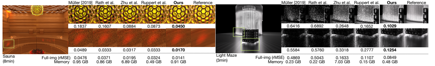
Fig. 10. Equal-time comparisons with some best performing baseline methods [Müller 2019; Rath et al. 2020; Ruppert et al. 2020] on two complex-visibility scenes. The incident radiance fields of these scenes contain high-frequency details and repeated patterns. We can still achieve better results in such light transport scenarios.
